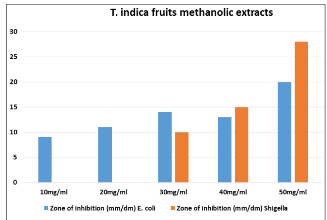
Fig 1: Graphical illustration of the antibacterial actions of T. indica fruits methanolic extracts
